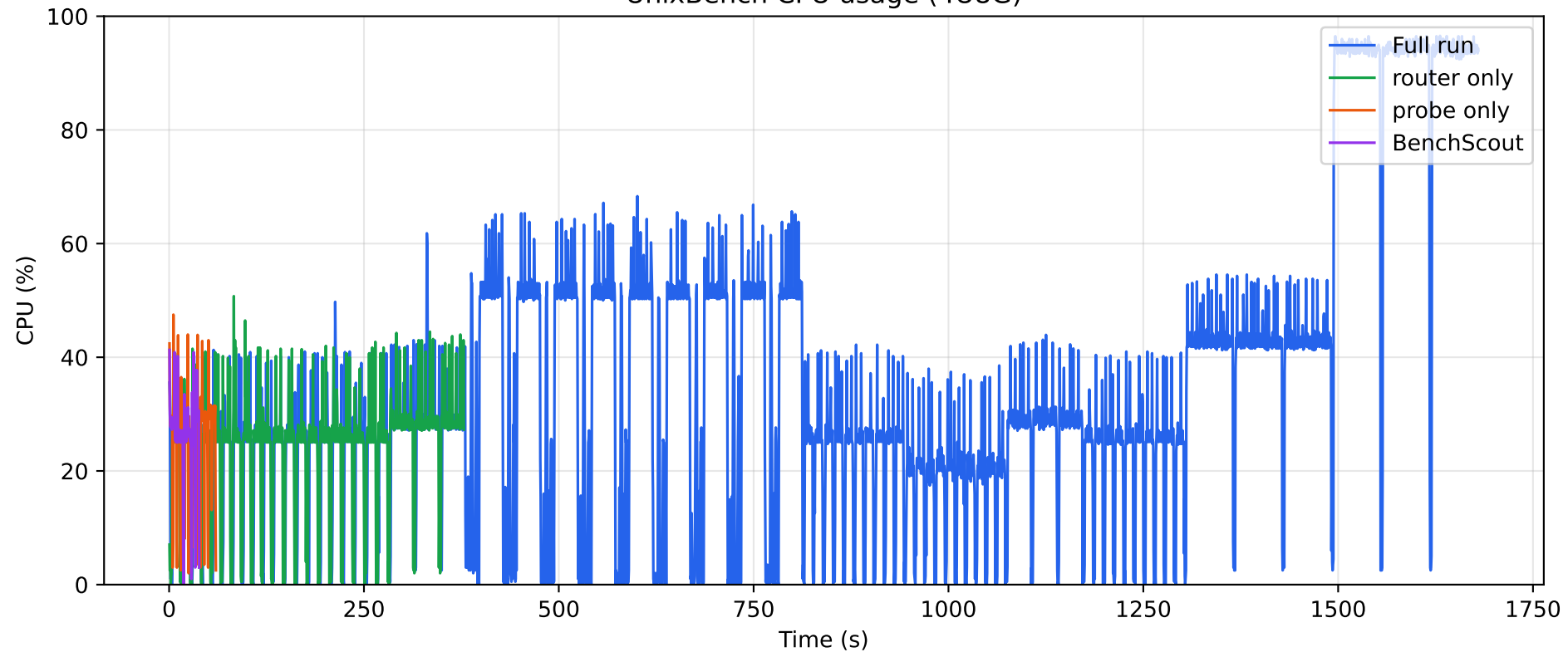
UnixBench CPU usage (4U8G)
