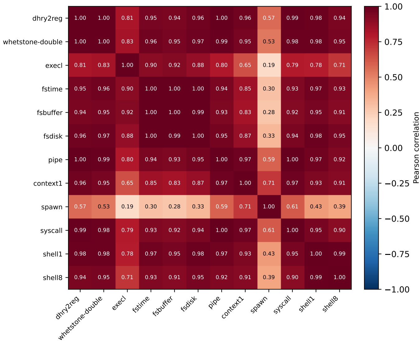
UnixBench subtest score correlation (Pearson, n=25 full runs)
