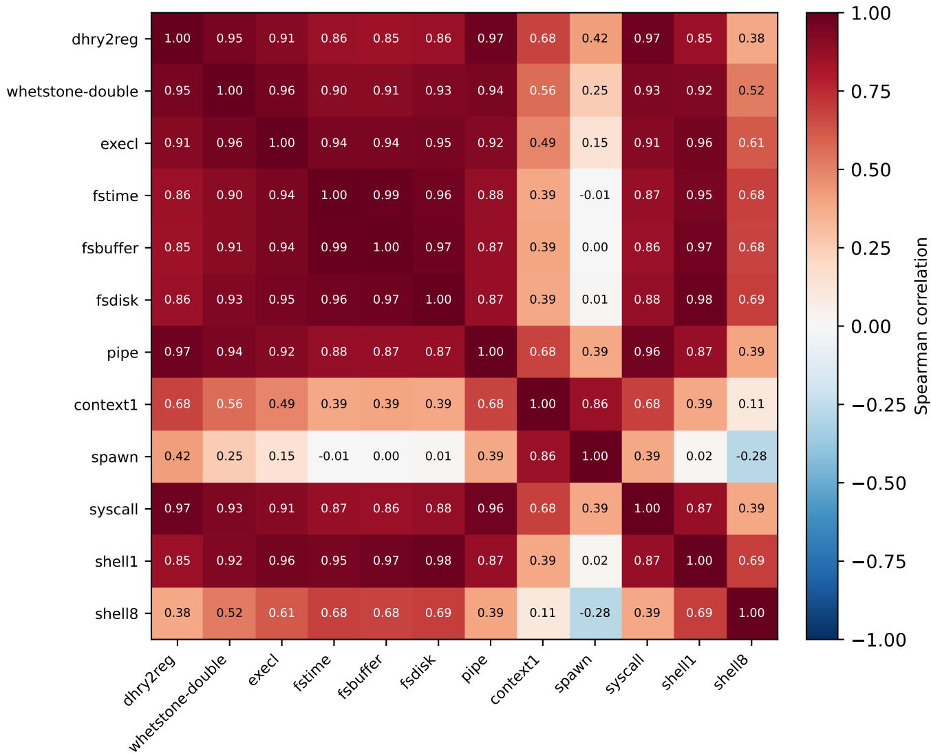
UnixBench subtest score correlation (Spearman, n=25 full runs)
