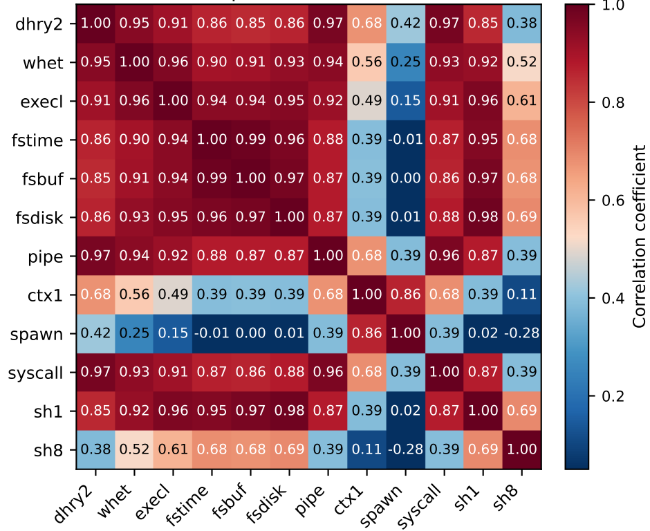
Spearman (n=25)
