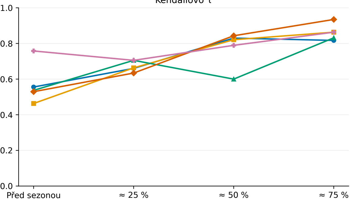
Kendallovo \tau
