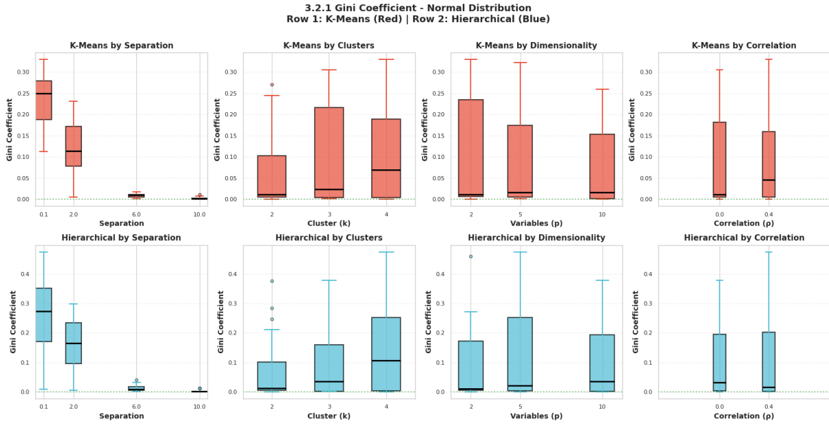
Figure 4.7: Absolute Gini Coefficients (Normal Distribution). Row 1: K-Means (Red). Row 2: Hierarchical Clustering (Blue). The metric approaches zero as separation increases, indicating balanced detection.
