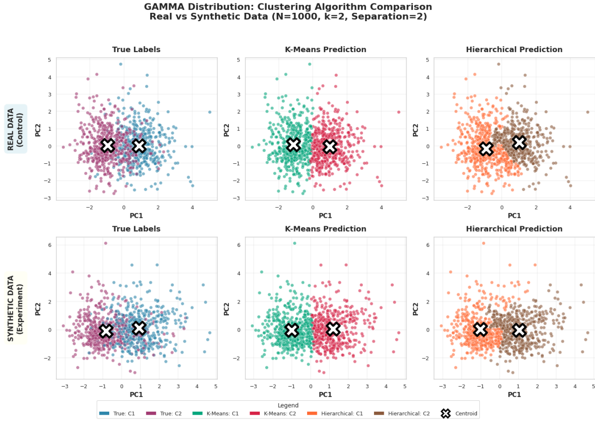
Figure 4.2: PCA Projection: Gamma Distribution ( N = 1000 , k = 2 ). Comparison of Real (Top) vs. Synthetic (Bottom). In the lower-left panel, “True Labels” denotes simulation-side diagnostic colouring only and does not imply observable labels or recordwise correspondence in practice.
