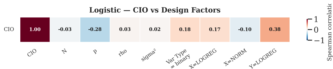
Figure 9.3: Spearman correlation heatmap between design factors and CIO for Logistic Regression. Source: Compiled by the author
