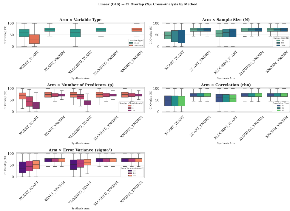
Figure 8.2: Comparison of CIO across synthesis methods (CART vs. Parametric) for Linear Regression. Source: Compiled by the author
