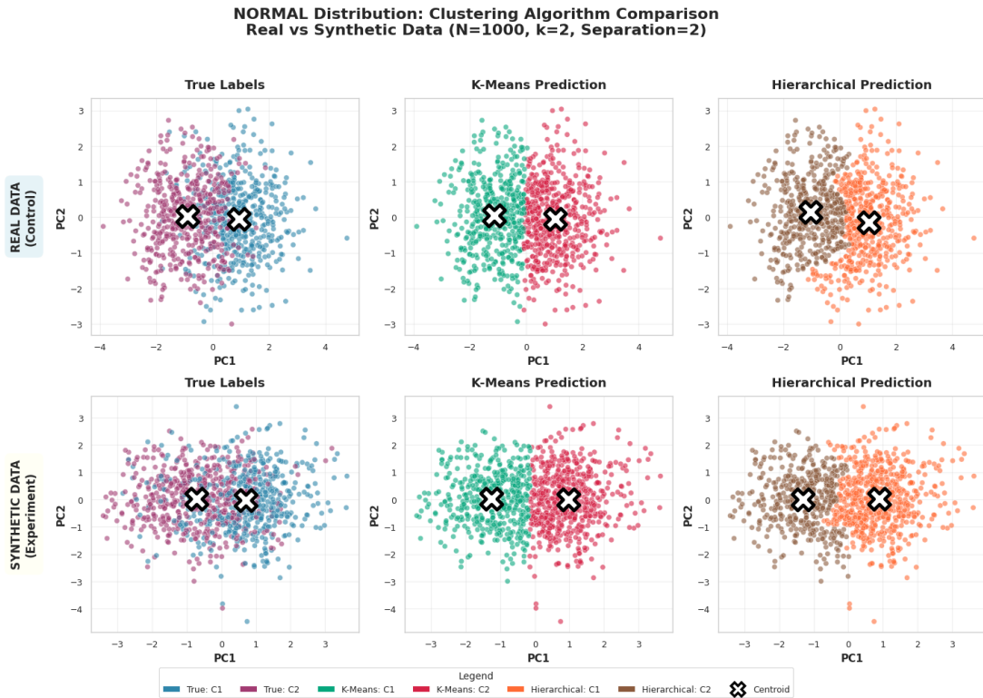
Figure 4.1: PCA Projection: Normal Distribution ( N = 1000, k = 2 ). Comparison of Real (Top) vs. Synthetic (Bottom).
