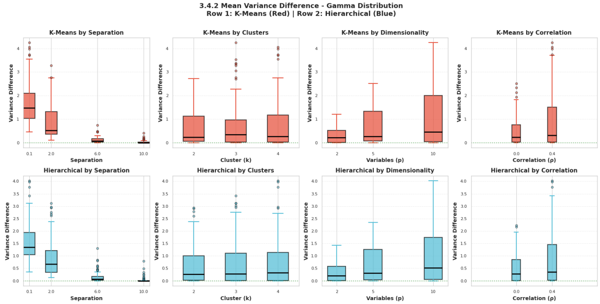
Figure 4.12: Mean Variance Difference (Gamma Distribution) . Row 1: K-Means (Red). Row 2: Hierarchical Clustering (Blue). Similar to the Normal case, variance distortion peaks in high-dimensional and correlated settings.
