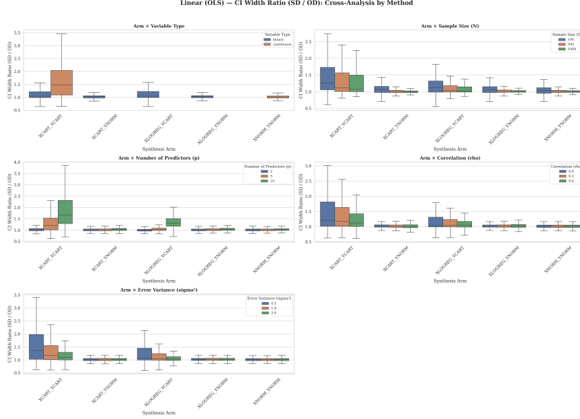
Figure 8.5: Distribution of the Confidence Interval Width Ratio by synthesis method for Linear Regression.
