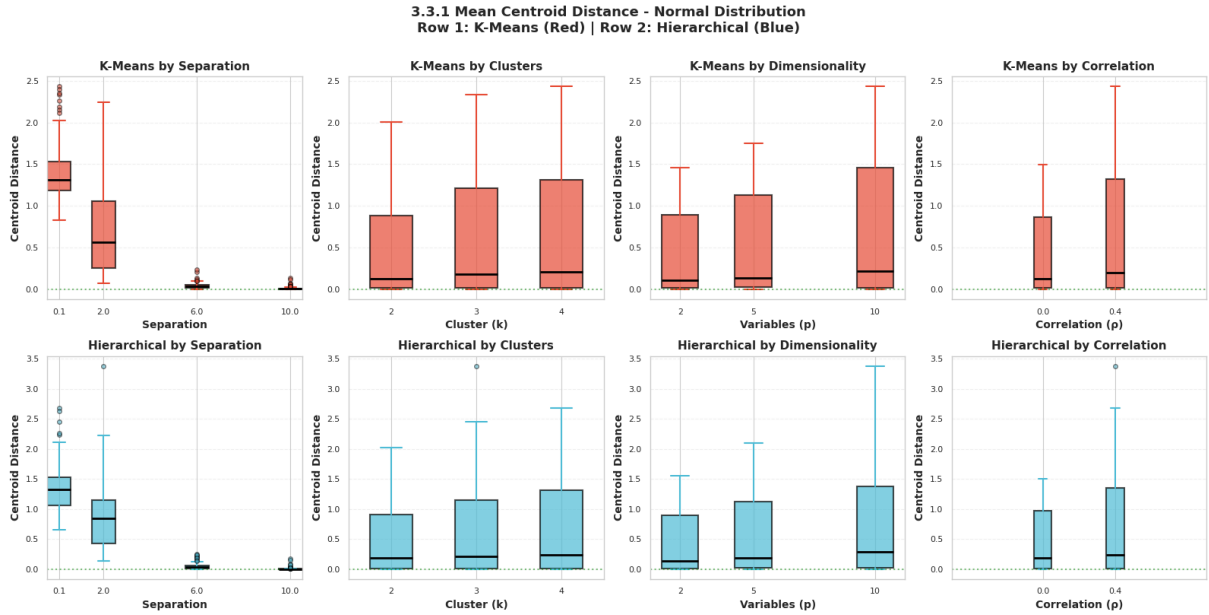
Figure 4.9: Mean Centroid Distance (Normal Distribution) . Row 1: K-Means (Red). Row 2: Hierarchical Clustering (Blue). The metric quantifies the Euclidean shift of cluster centers after synthesis.
