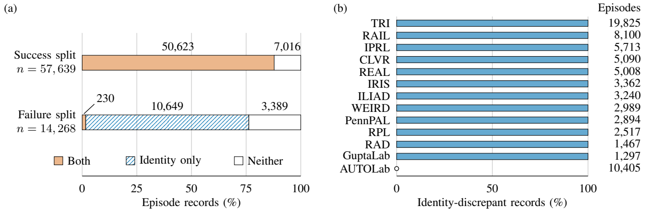
Fig. 3. Summary-layer audit of the pinned Cosmos3-DROID release. (a) Joint outcomes of identity-summary and task-text relations: both discrepant, identity only, or neither. Task-only discrepancies are zero. Success/failure are dataset outcome splits, not audit verdicts; labels give exact record counts. (b) Identity-discrepancy rates by the 13 source prefixes parsed from episode identifiers, combining both splits (ties ordered by episode count). These are source groups, not an independently verified inventory of laboratories. AUTOLab has zero discrepancy; the other 12 groups have 100%. These relations do not evaluate visual content or downstream harm.
