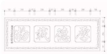
Figure 3: Plaque component instance.
