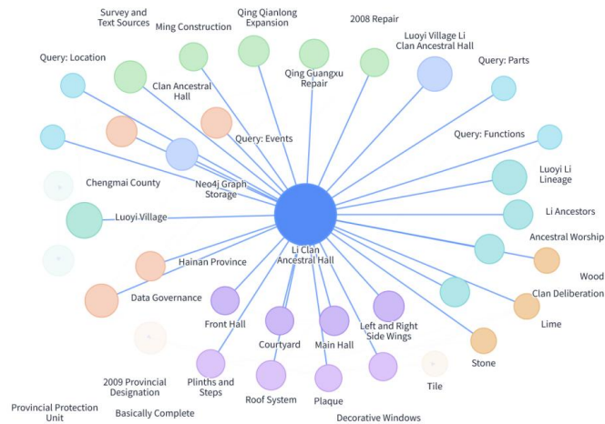
Figure 5: The constructed knowledge graph.
