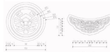
Figure 4: Cylindrical tile and drip-tile component instances.
