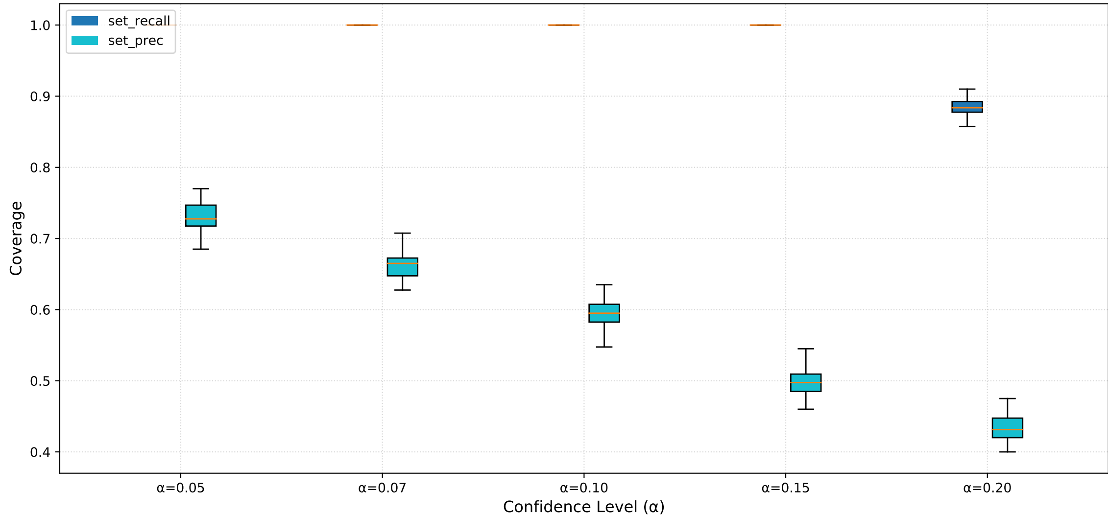
Coverage Across Methods and Confidence Levels
