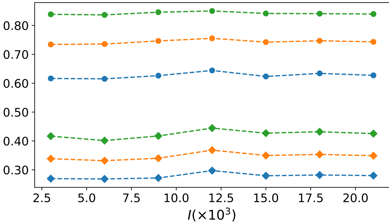
empirical power
