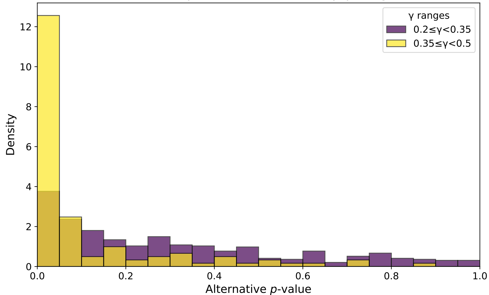
Alternative p -value Distributions by \gamma Ranges
