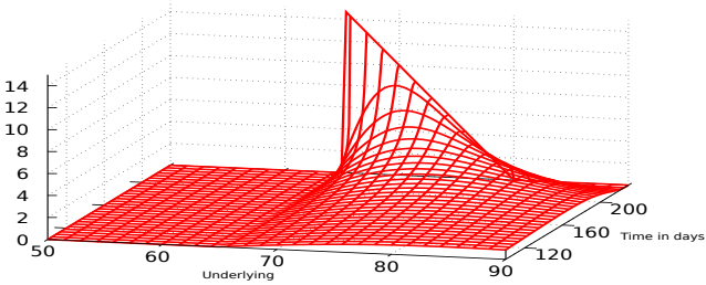
Fig. 11.16: Graph of the down-and-out put option price (11.12) with K = 80 > B = 65 .
