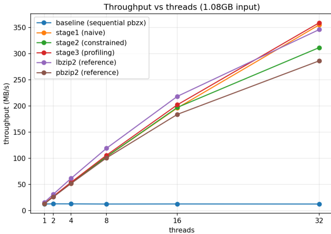
Fig. 2. Throughput (MB/s) vs. thread count for all five parallel implementations and the sequential baseline on the 1.08GB input.
