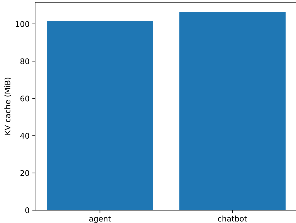
Mean per-request peak KV-cache usage
