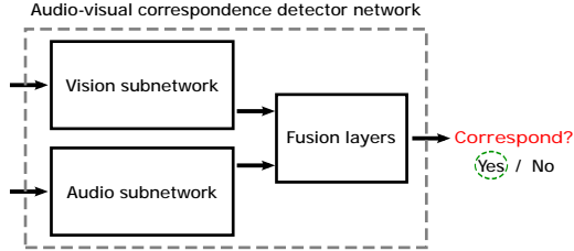
Figure 1. Audio-visual correspondence task (AVC). A network should learn to determine whether a pair of (video frame, short audio clip) correspond to each other or not. Positives are (frame, audio) extracted from the same time of one video, while negatives are a frame and audio extracted from different videos.
