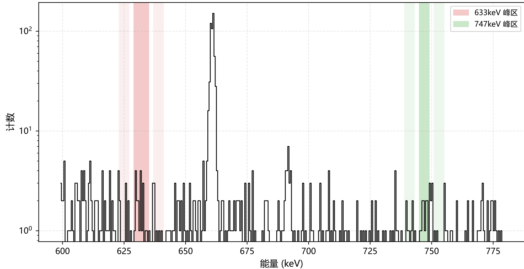
HPGe 谱与峰积分窗口 —— 10.11Co57.Spe
