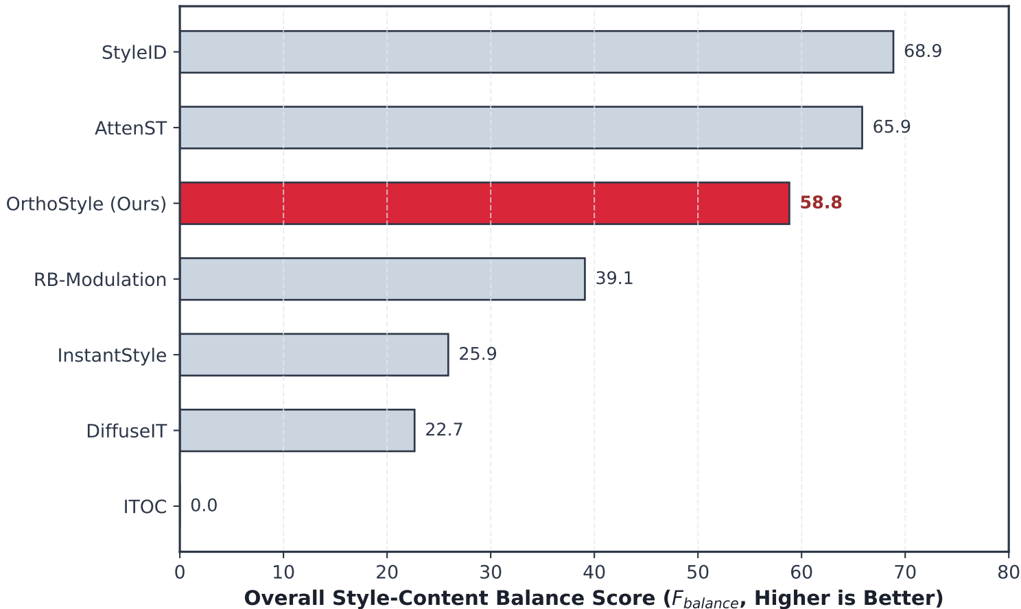
Overall Style-Content Balance Score (Harmonic Mean)
