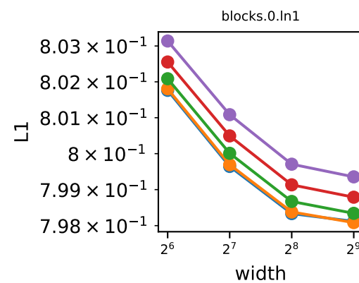
μP coord check — L1 of module outputs vs width
