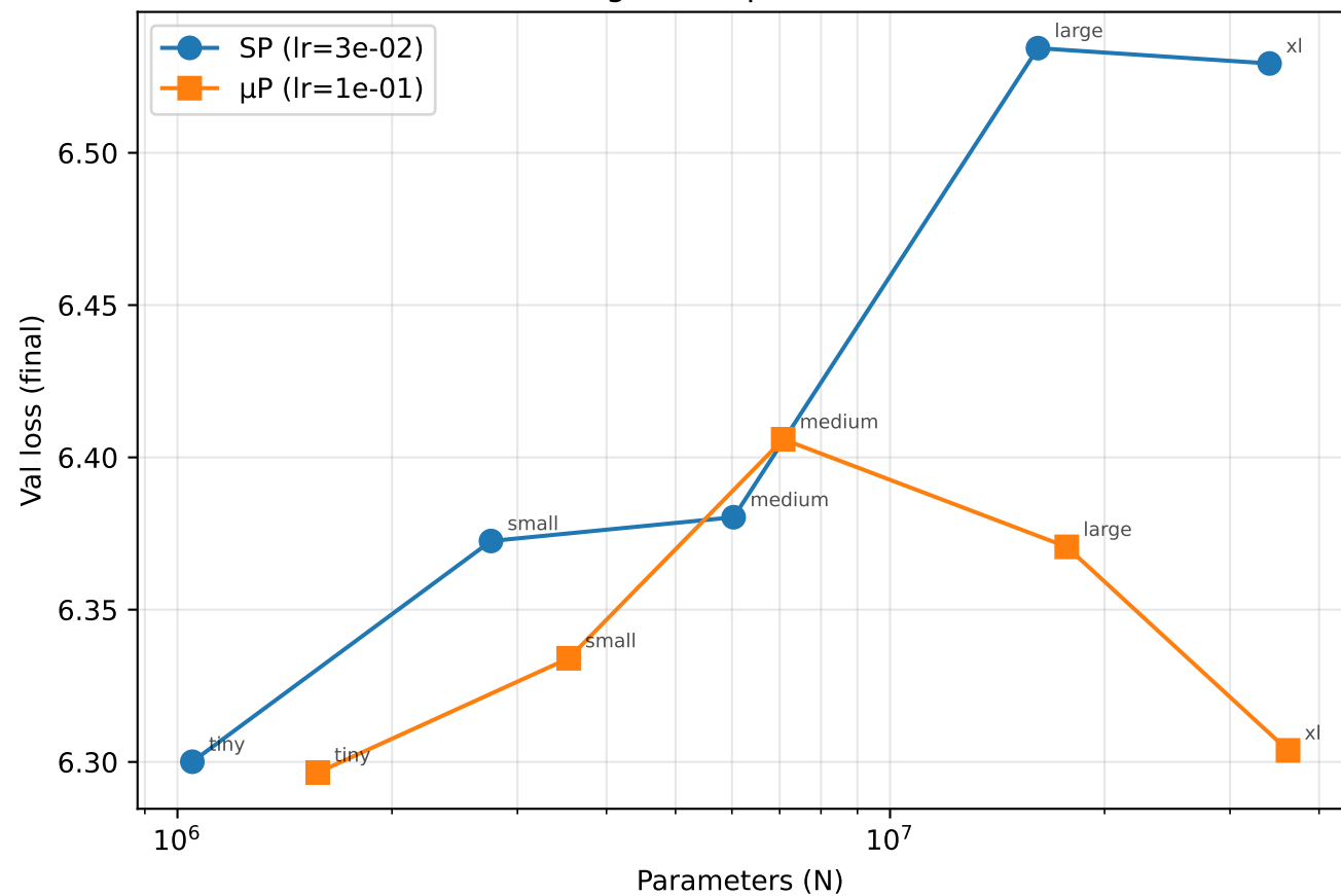
Scaling: SP vs \mu P at fixed LR
