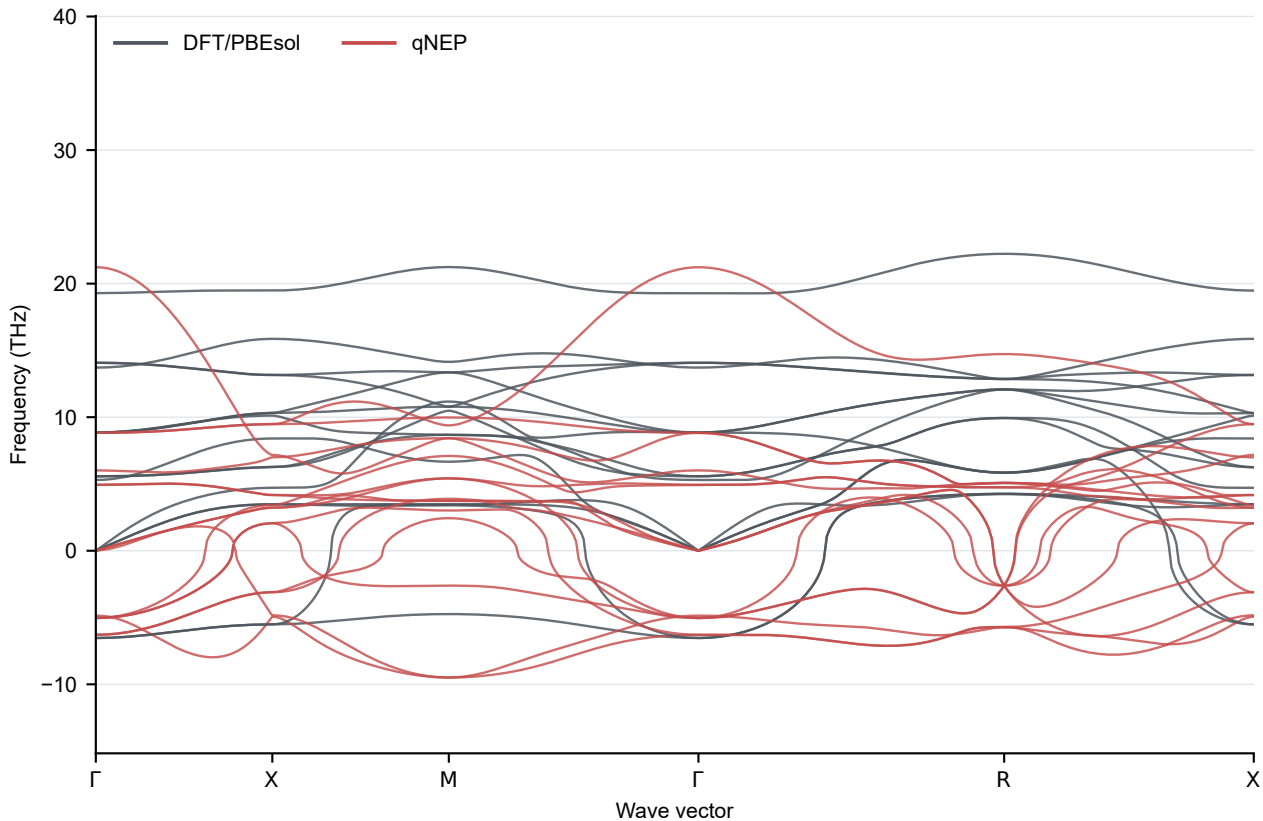
Cubic BaTiO 3 : DFT vs qNEP with NAC
