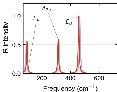
(e) — ZStar (VASP) — Ref. [83]
