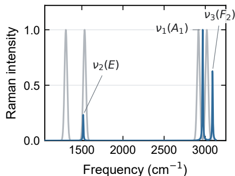
(l) — ZStar — Ref. [84]
