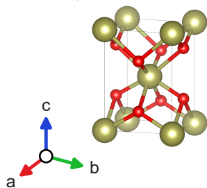
(a) HfO 2 3D, bulk
