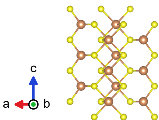
(g) Sb 2 S 3 1D, nanowire
