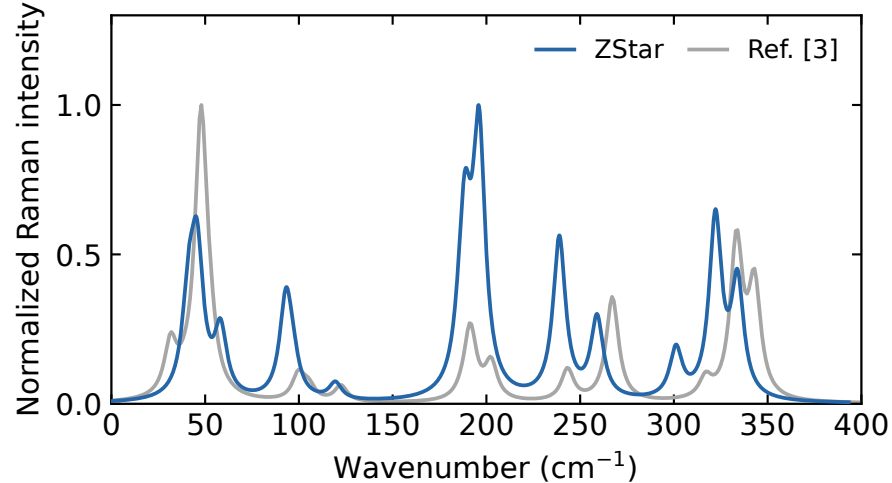
(f) \text{Sb}_2\text{S}_3 chain | Raman
