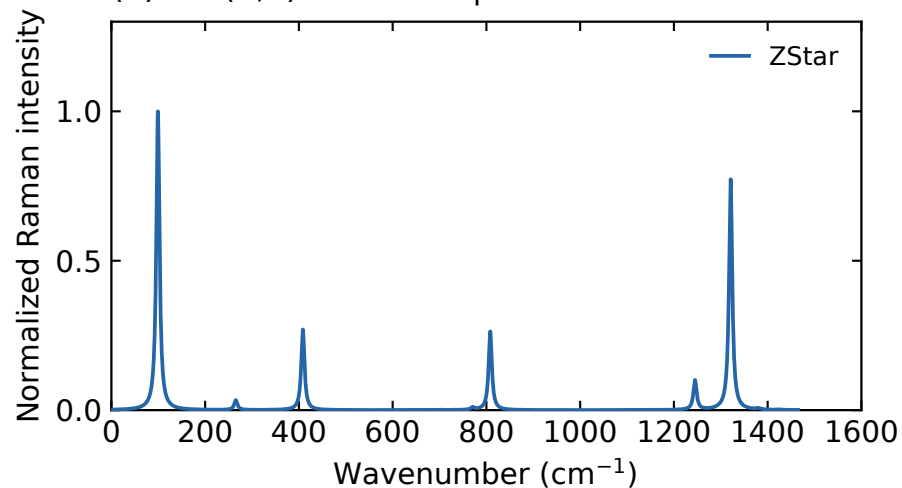
(b) BN(6,0) nanotube | Raman
