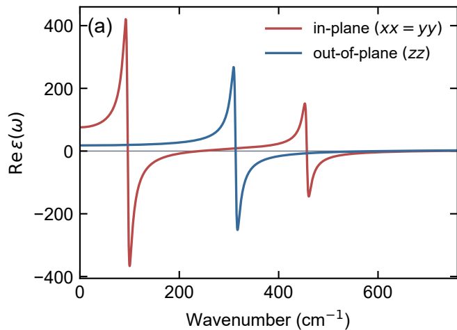
monolayer \text{MoS}_2 : lattice sheet response
