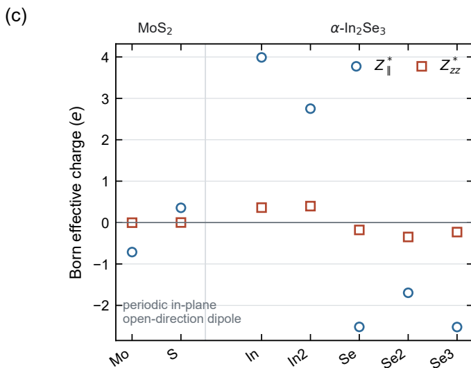
2D hybrid response: calculated representatives
