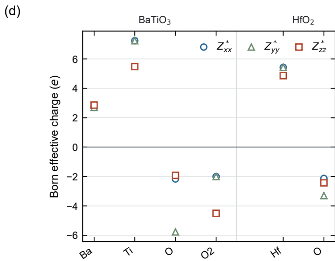
3D bulk response: calculated representatives
