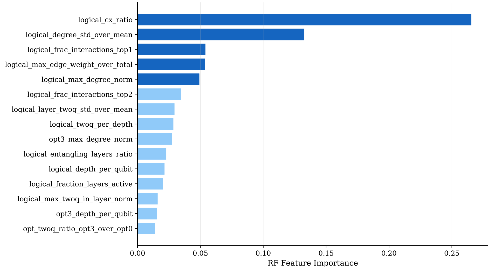
Top 15 features by RF importance (dark blue = top-5 used in ablation)
