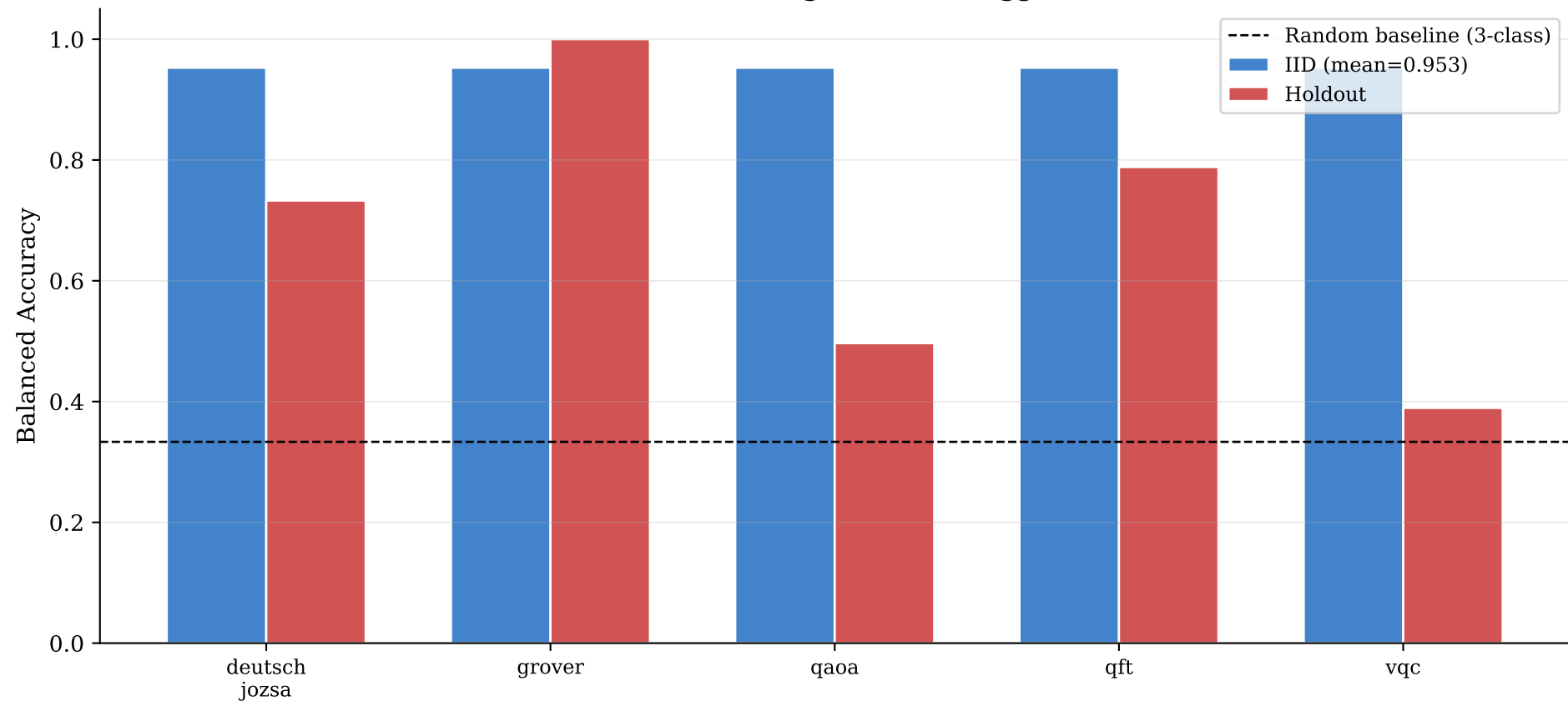
Random Forest: IID vs leave-one-family-out holdout (three-class: benign / static / triggered)
