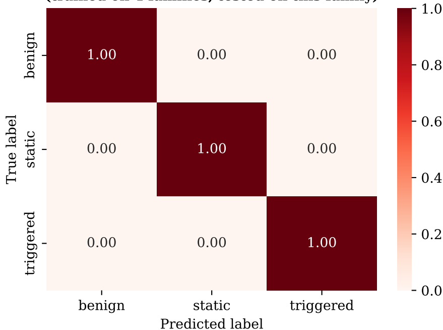
RF holdout — grover (trained on 4 families, tested on this family)
