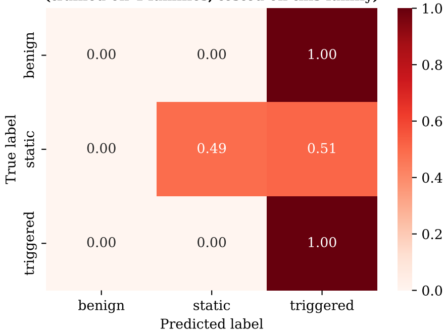
RF holdout — qaoa (trained on 4 families, tested on this family)
