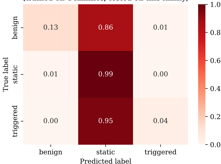
RF holdout — vqc (trained on 4 families, tested on this family)
