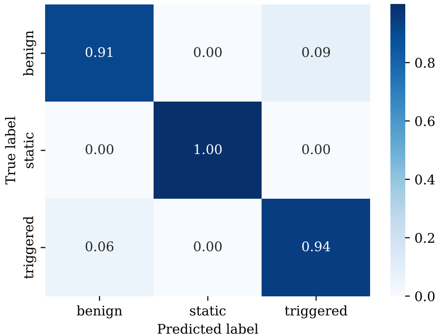
RF confusion matrix — IID (normalised)
