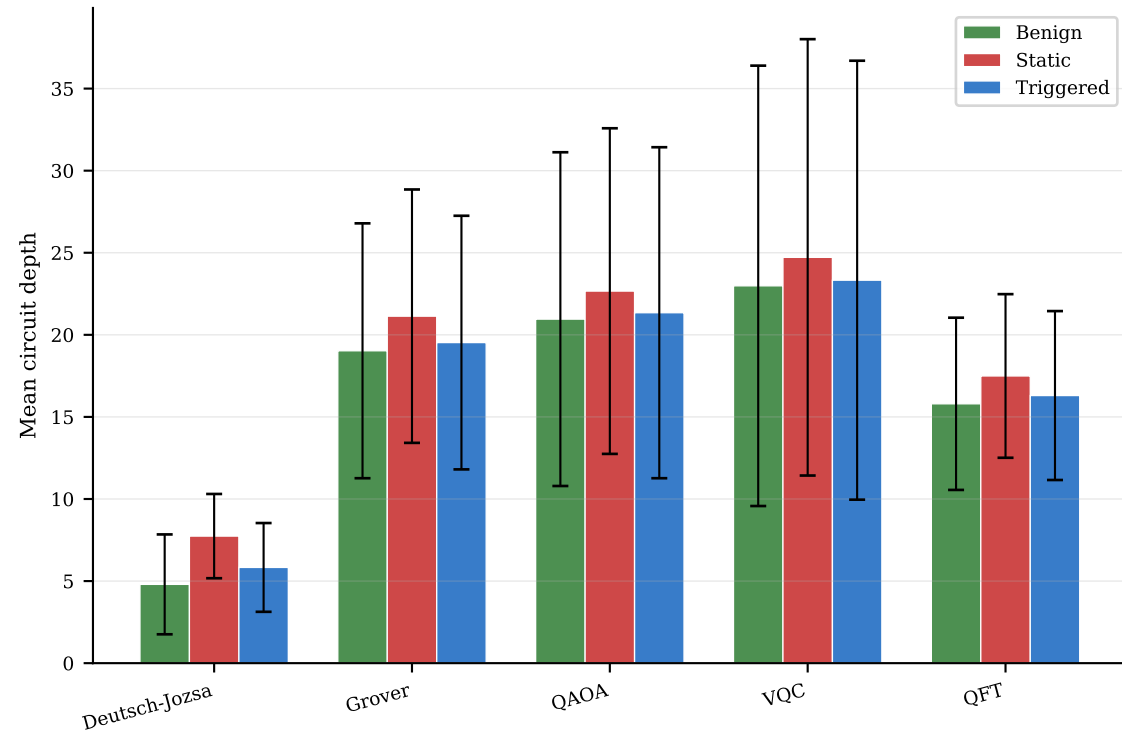
Circuit depth by class and family
