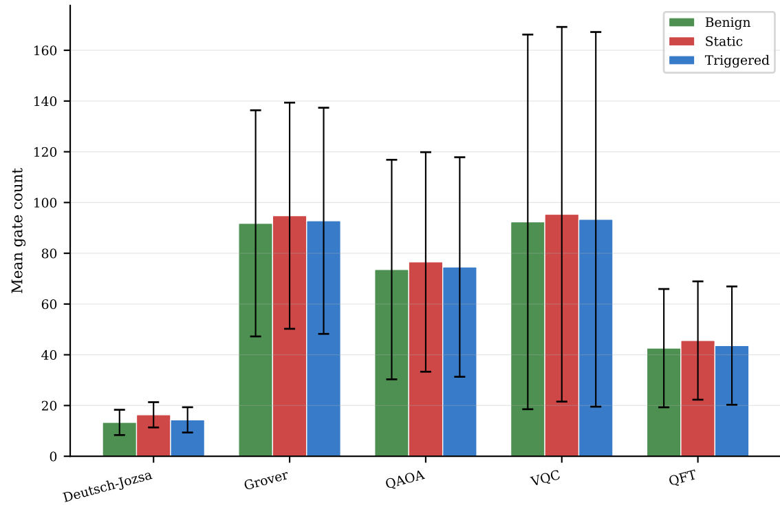
Gate count by class and family
