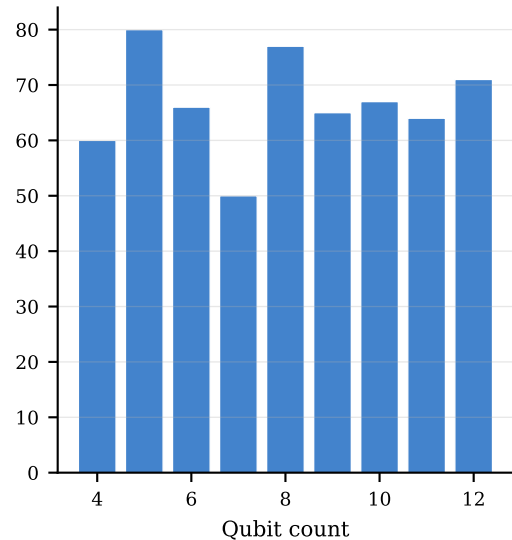
Grover
