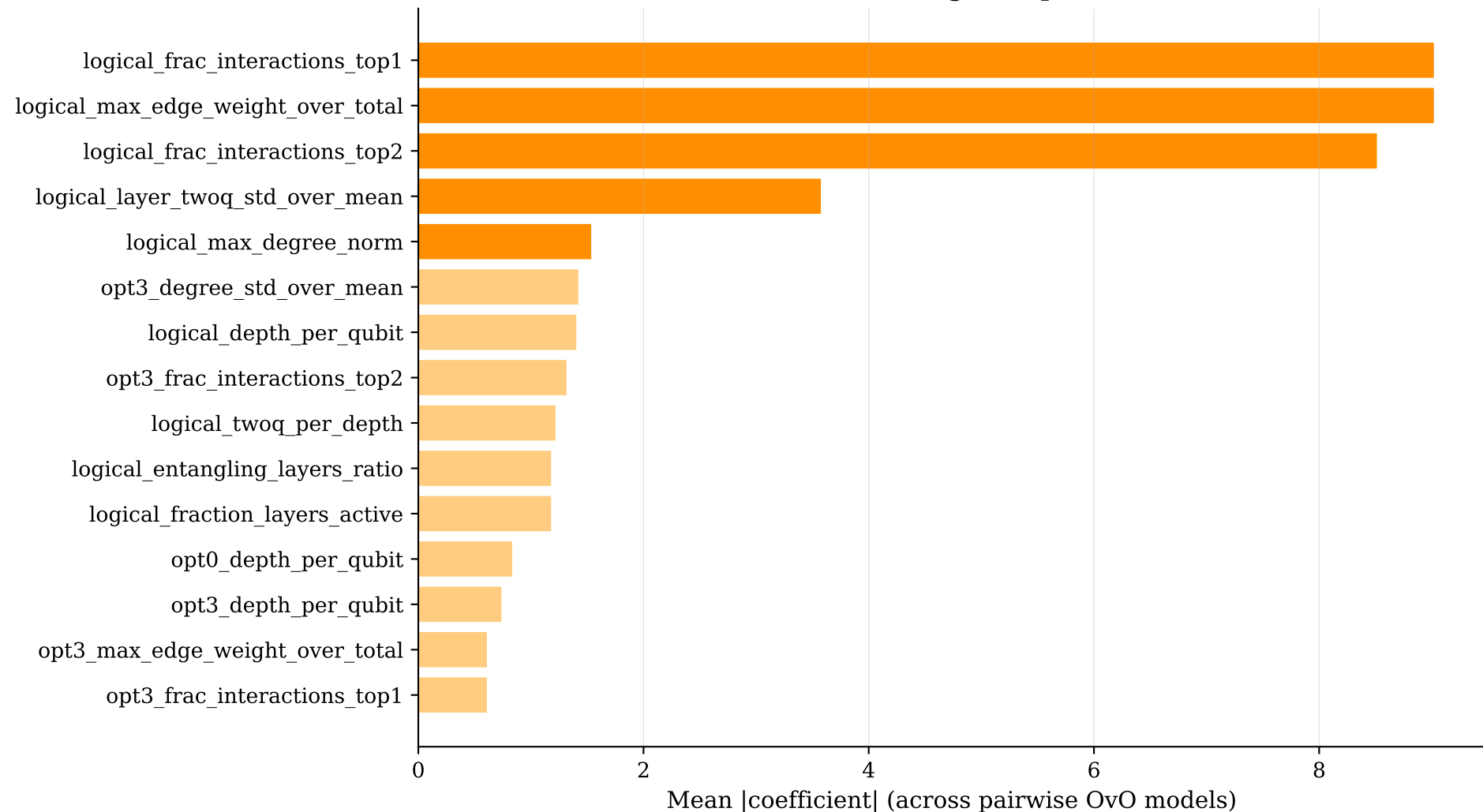
Top 15 features by linear SVM coefficient magnitude (dark orange = top-5)
