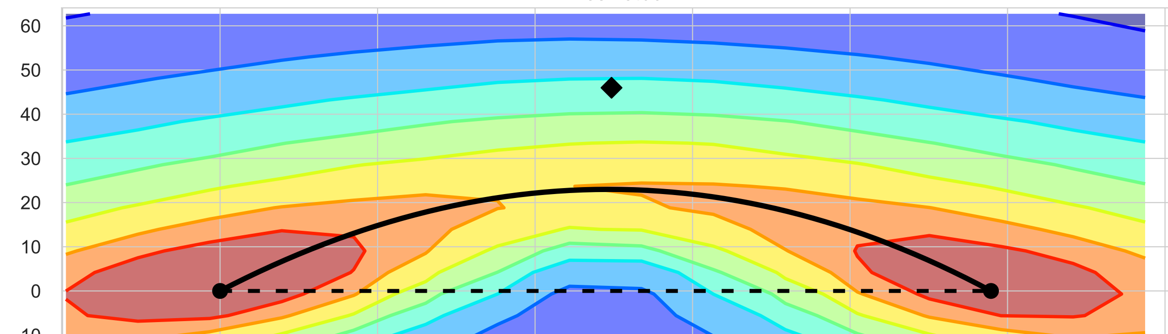
ResNet119
