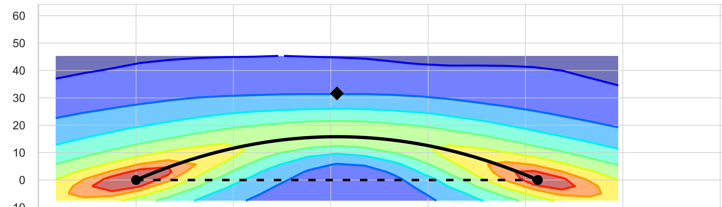
ResNet26
