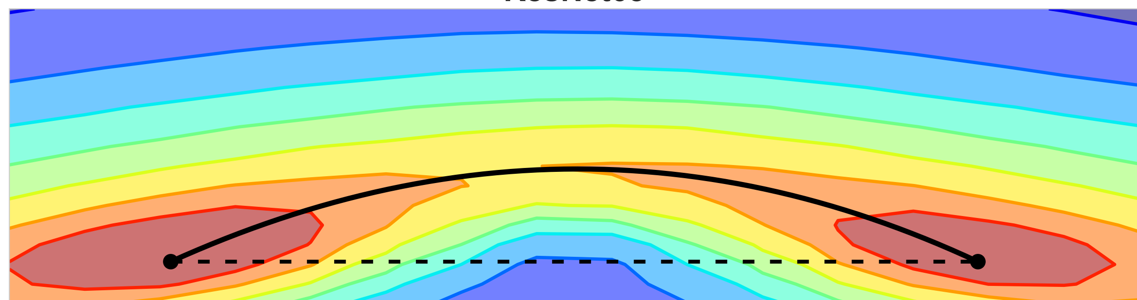
ResNet65
