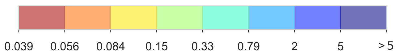
ResNet-8
