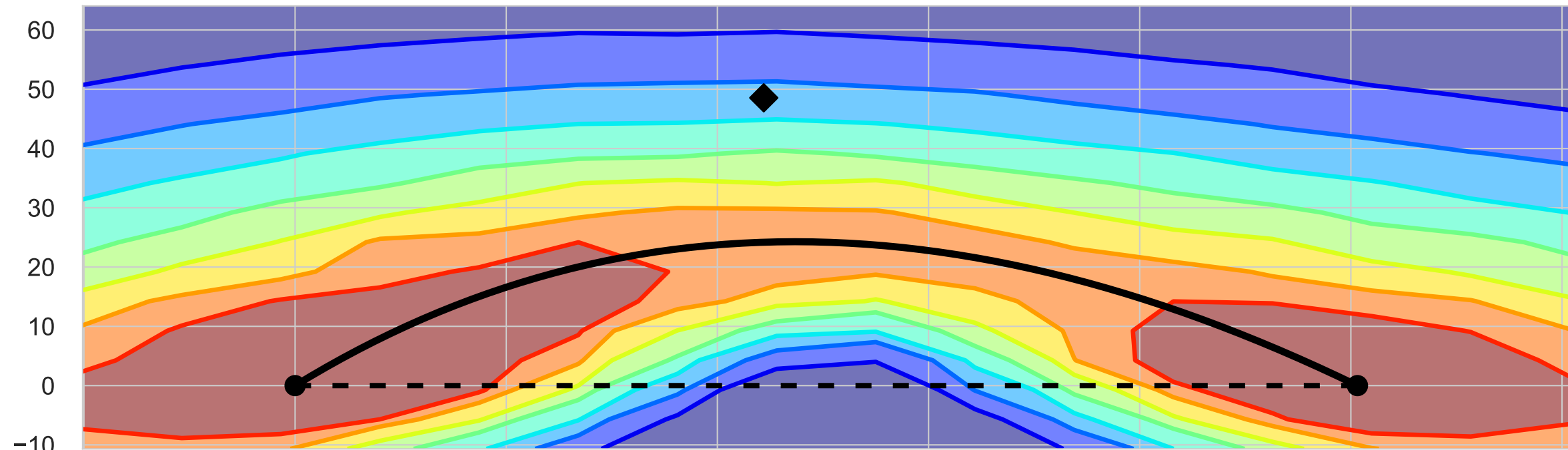
ResNet119
