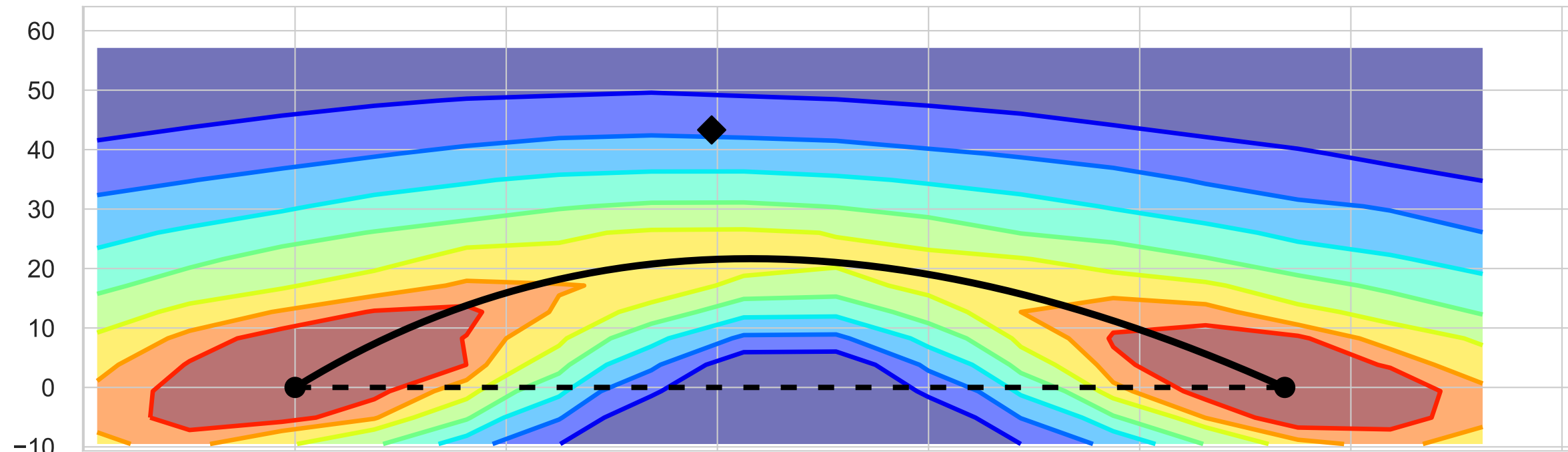
ResNet65
