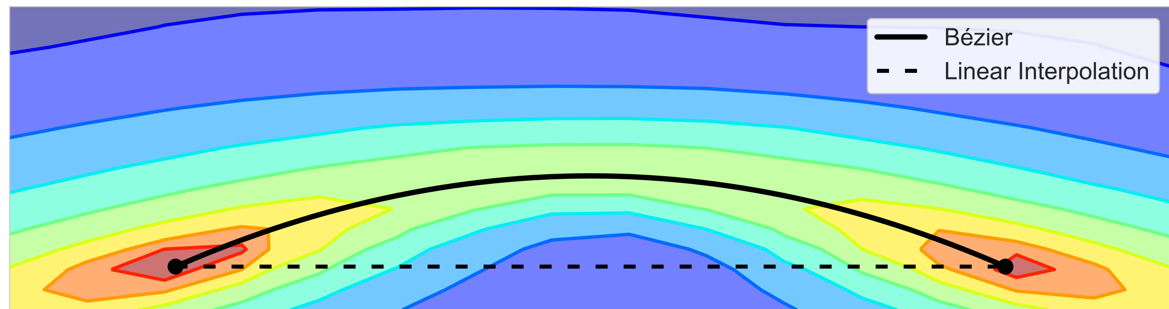
ResNet8
