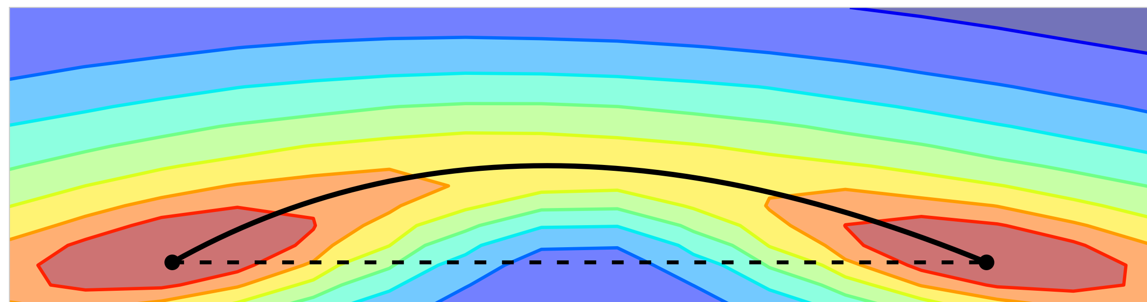
ResNet38
