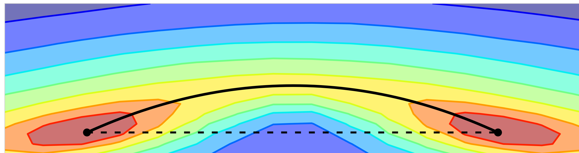
ResNet26
