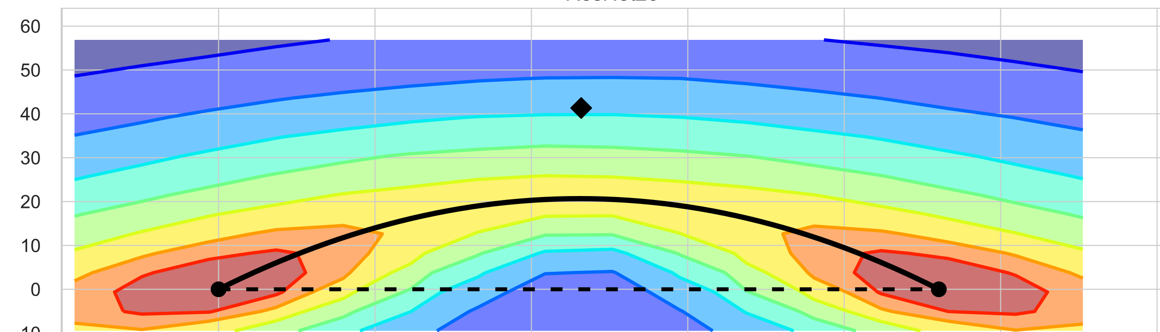
ResNet38
