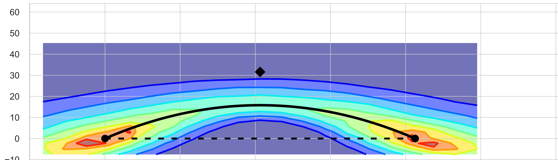
ResNet26
