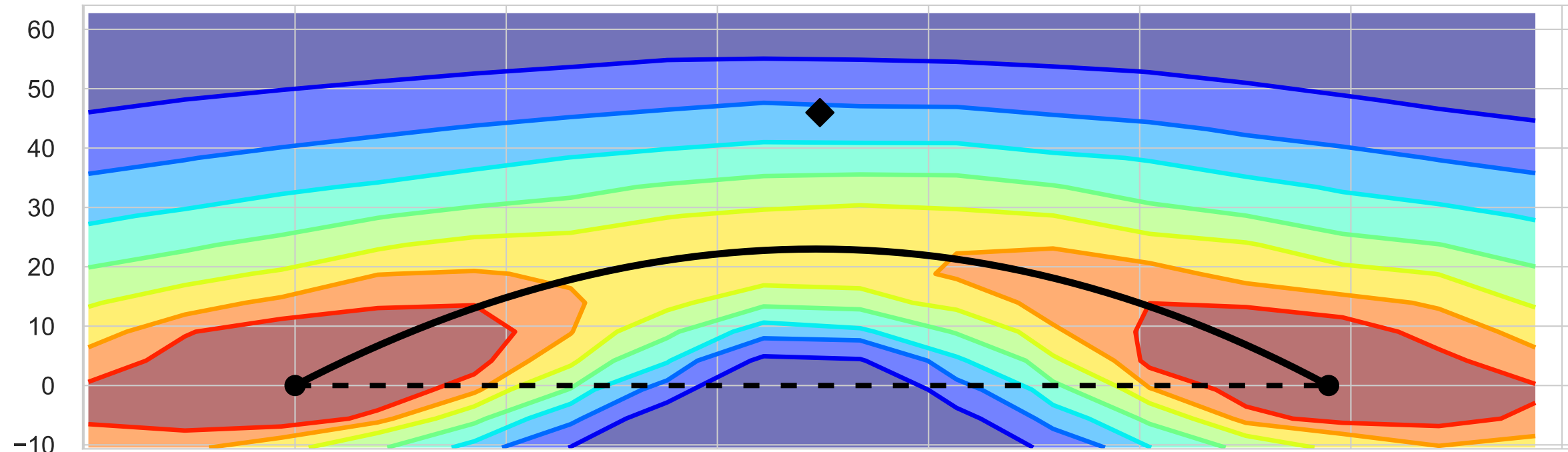
ResNet119
