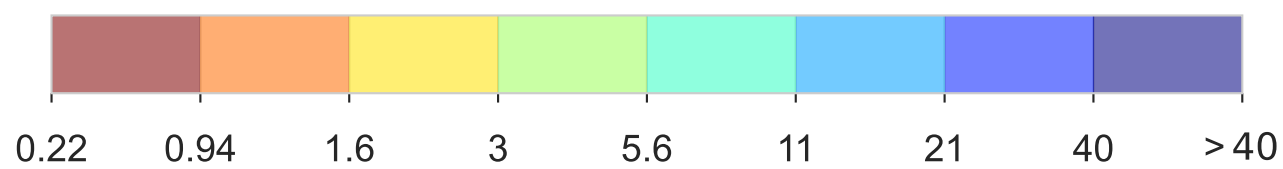
ResNet8
