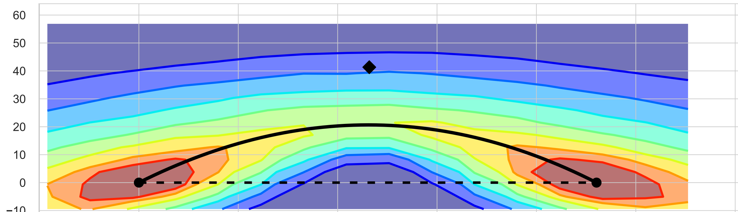
ResNet38
