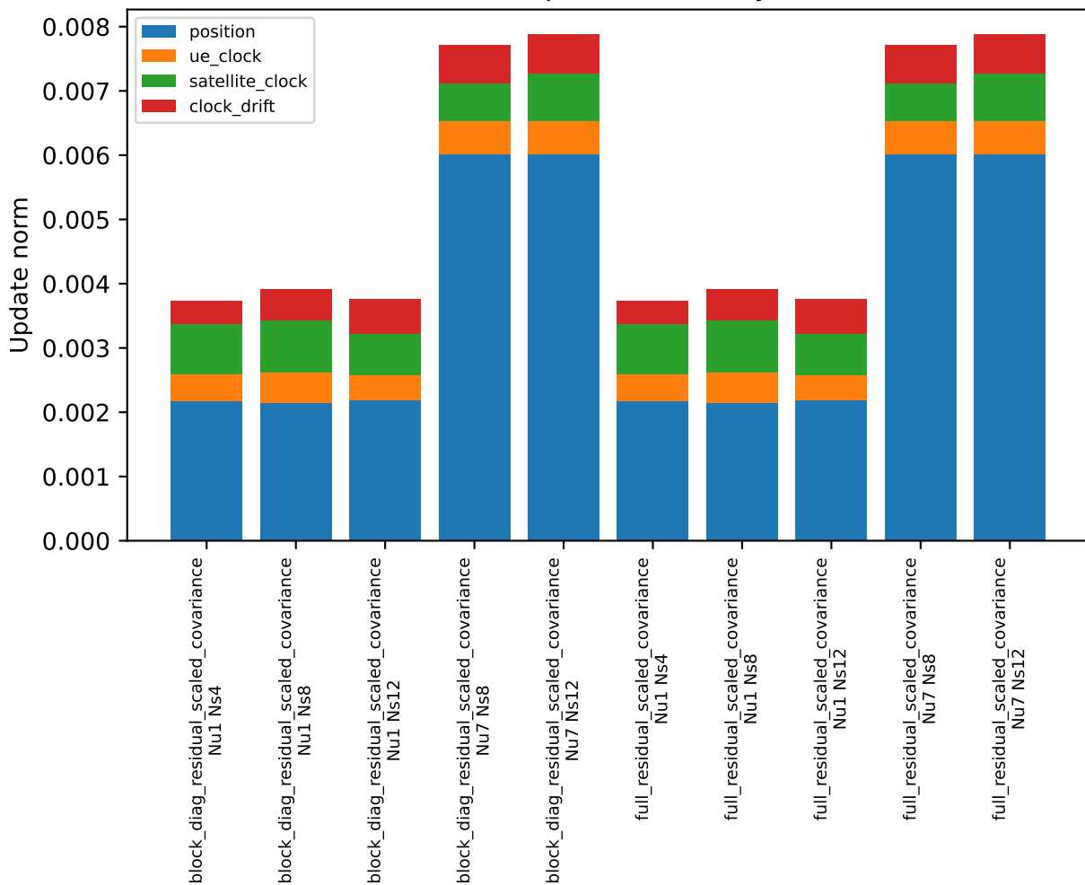
Failure-row update norms by block
