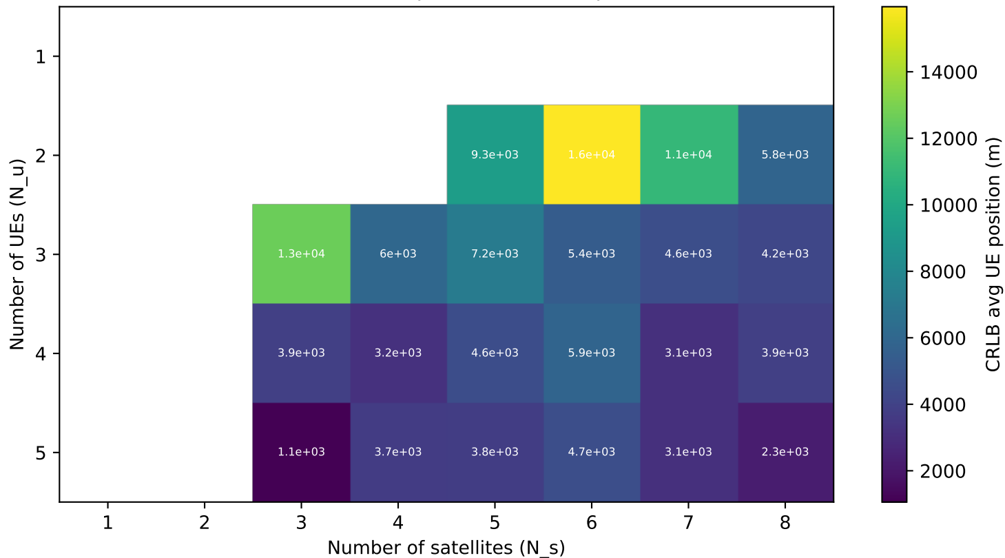
Wave CRLB position heatmap
