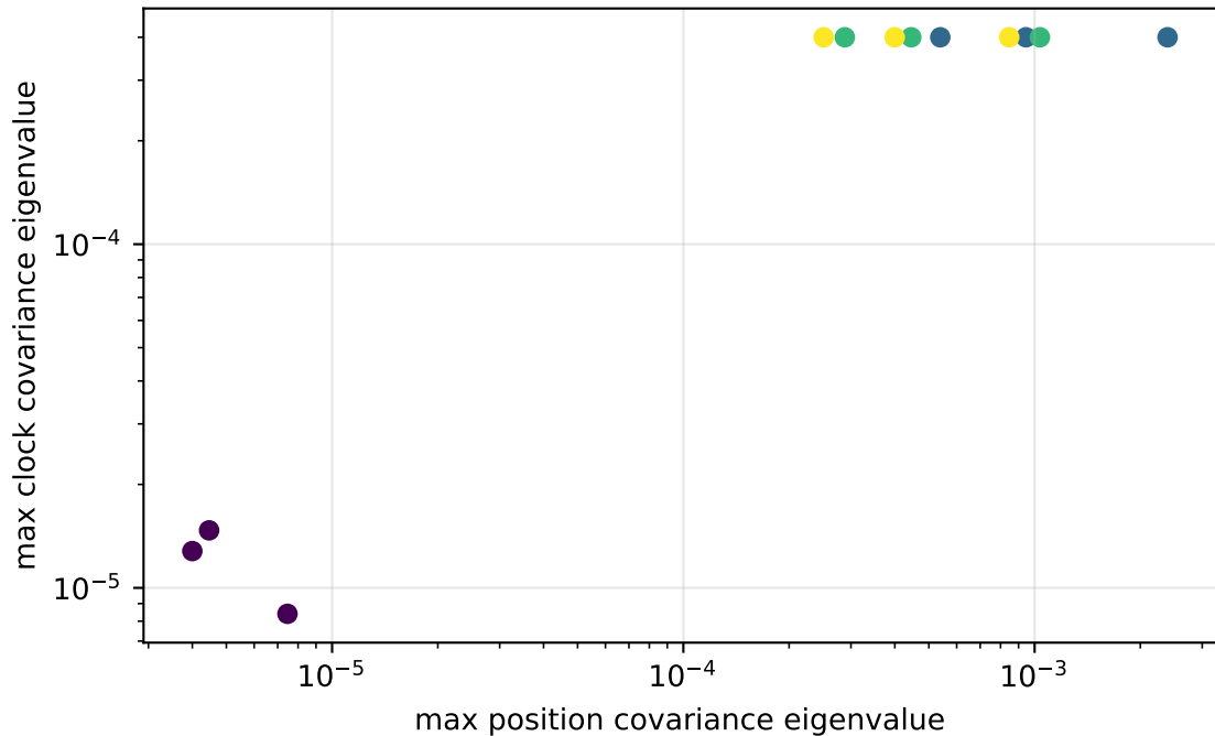
C7 covariance eigenvalue diagnostics
