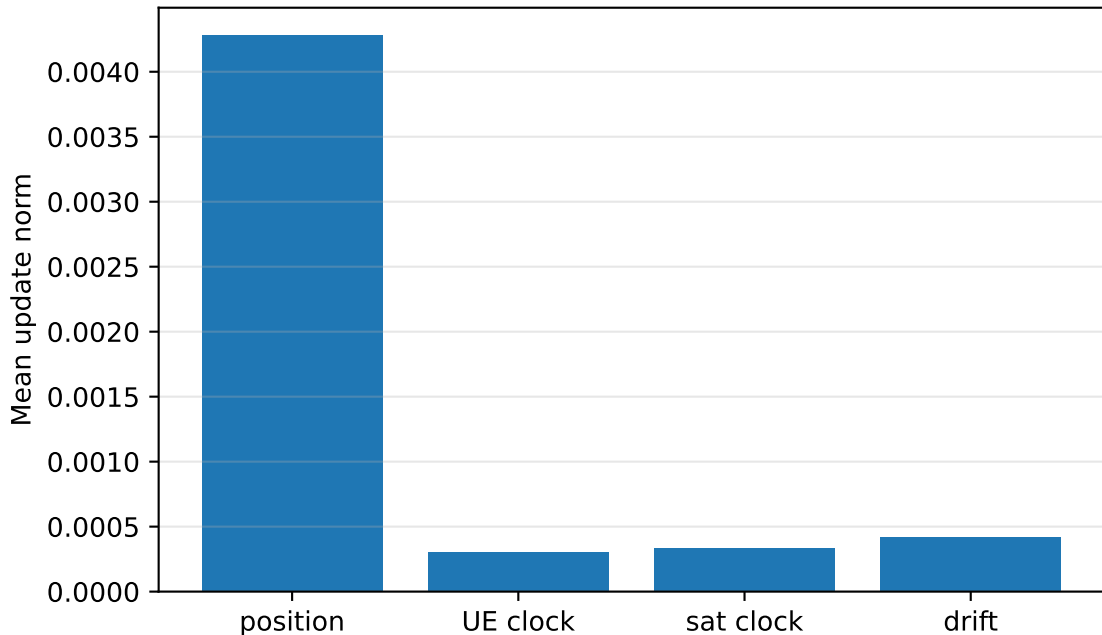
C7 update norm by state block
