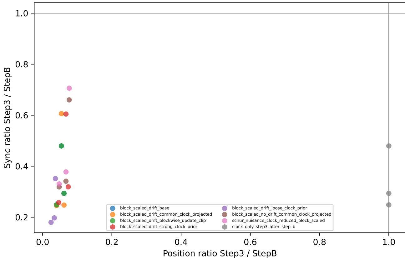
Sparse near-winner Step 3 variants
