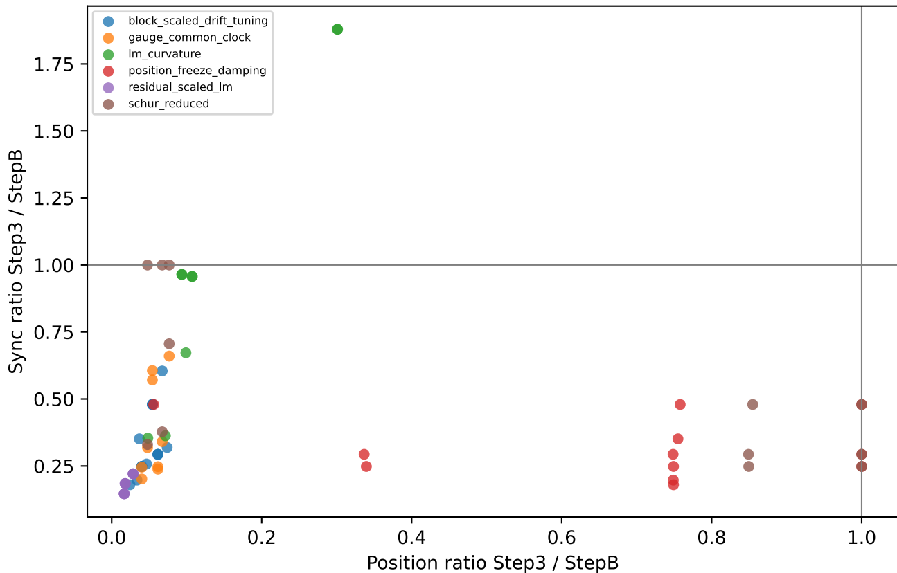
Step 3 covariance exploration
