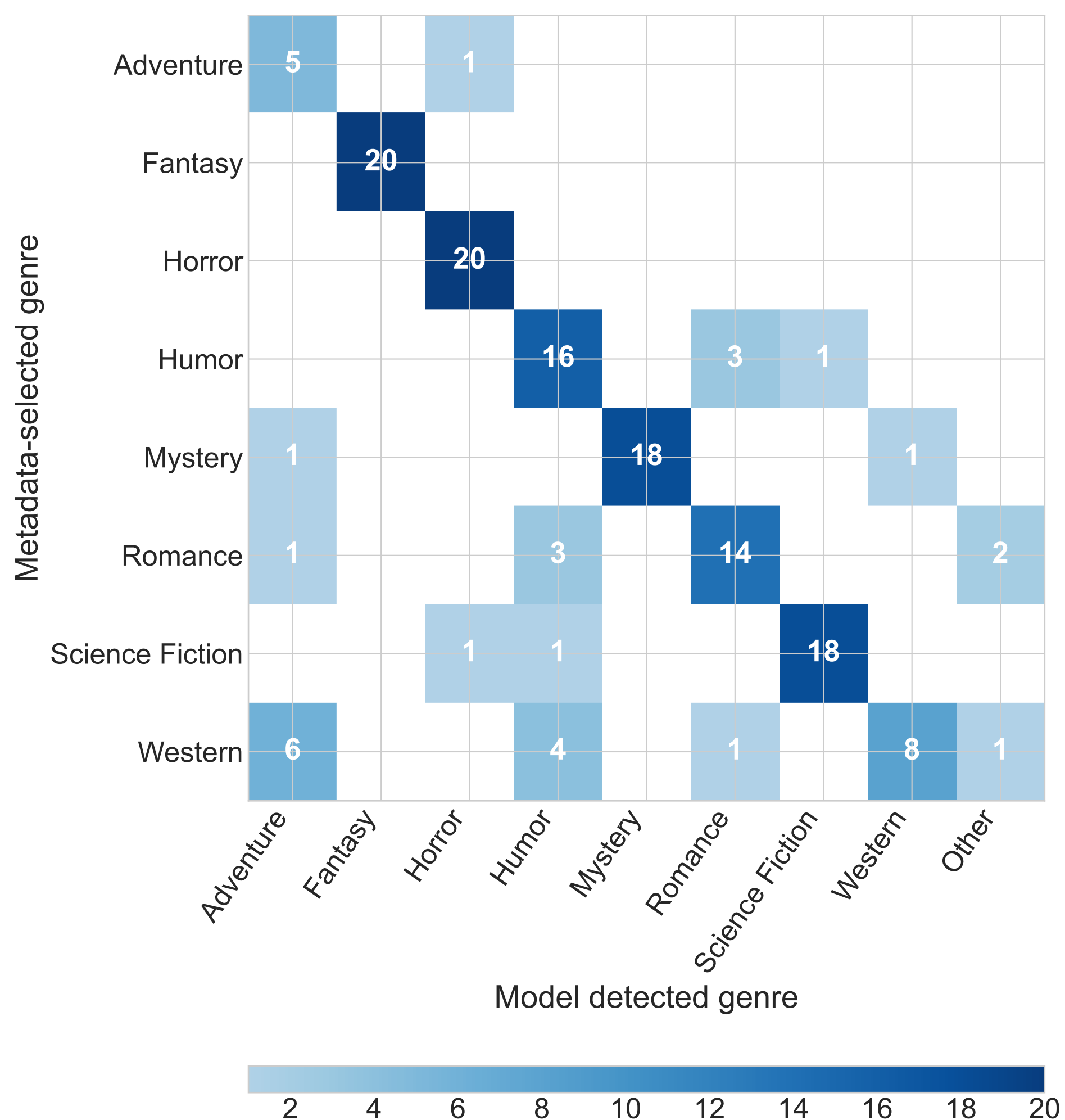
Metadata → Model Confusion
