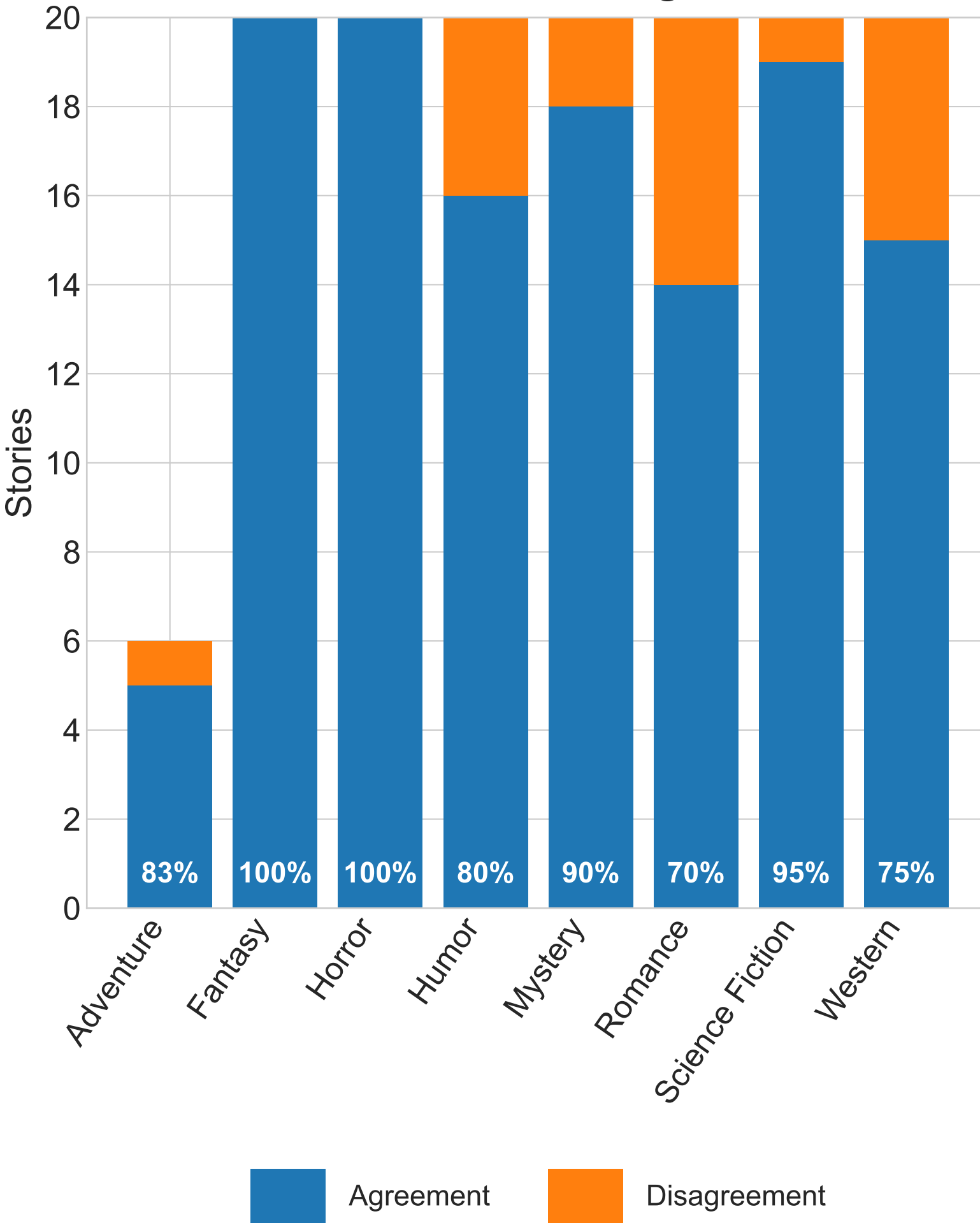
Metadata / Model Agreement
