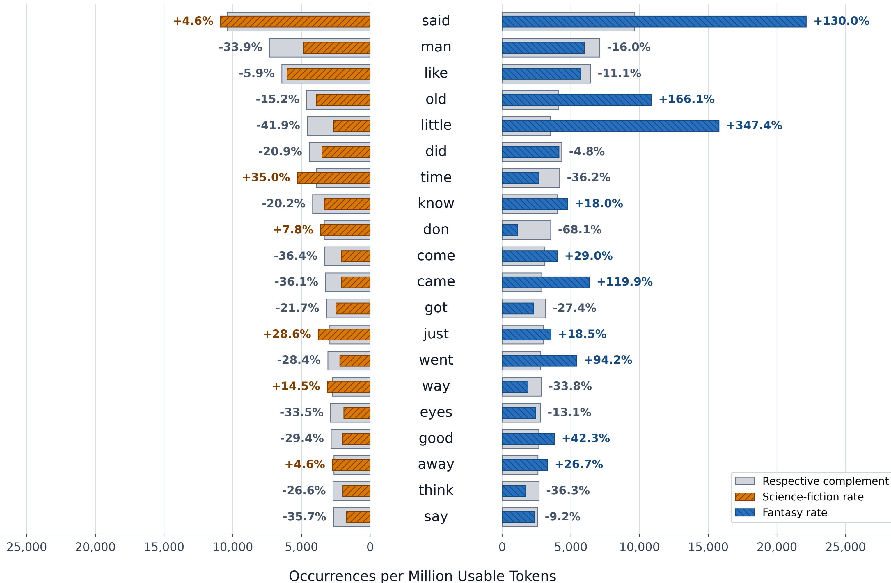
Science Fiction Relative to Baseline
