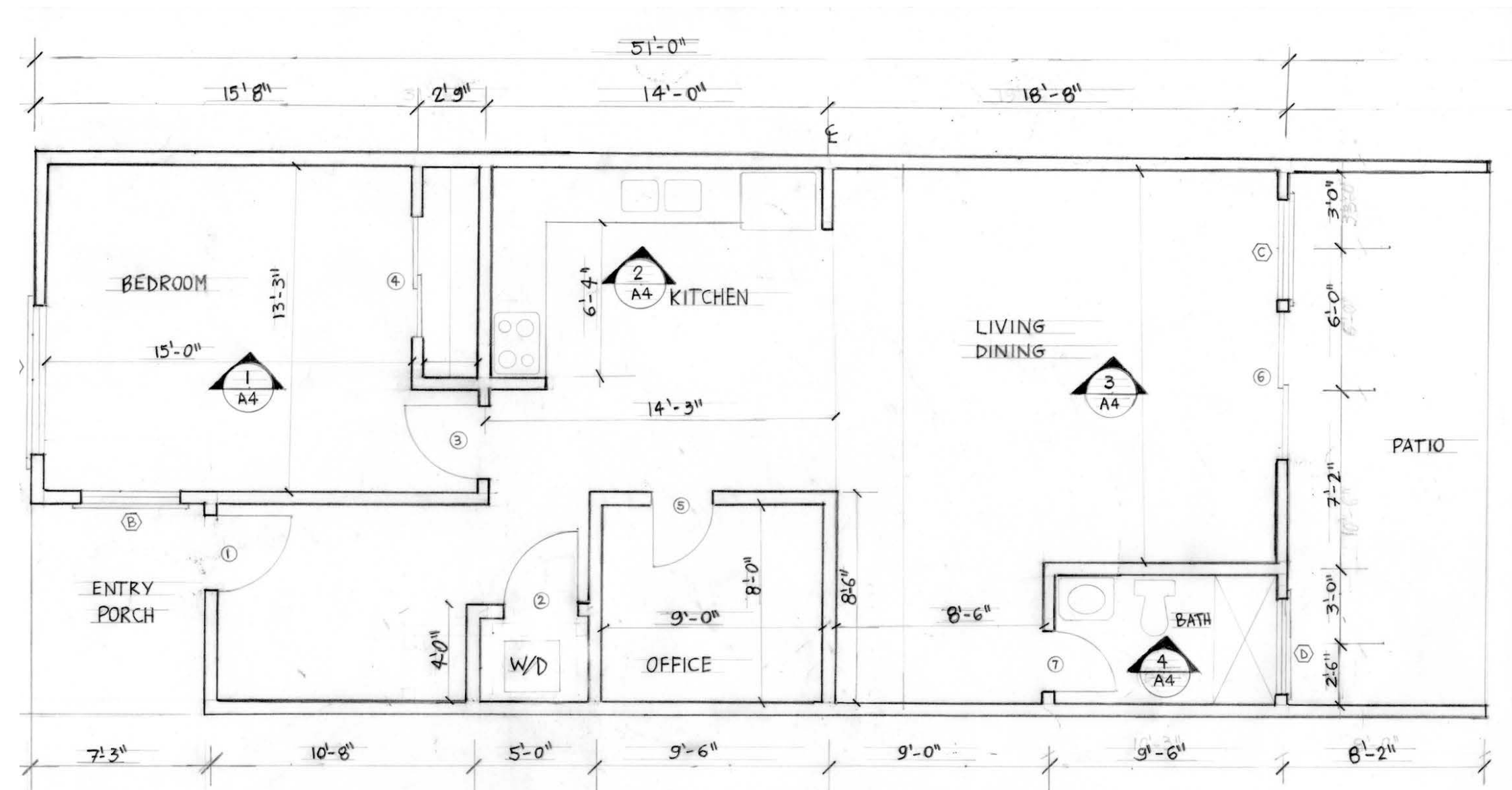
FLOOR PLAN
