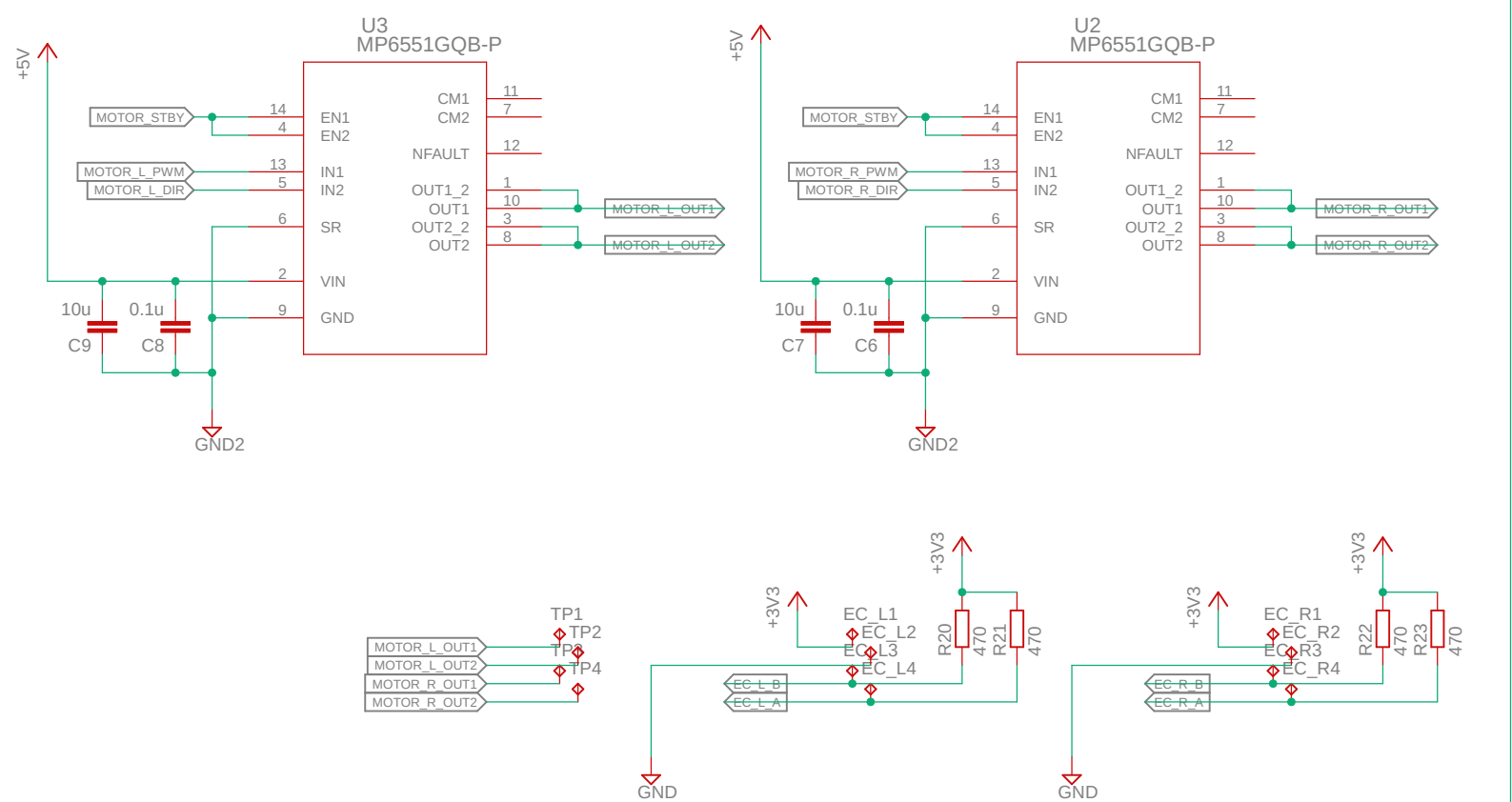
Motor Driver
