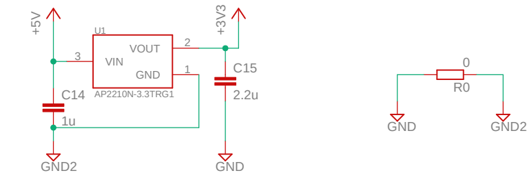
Power Supply
