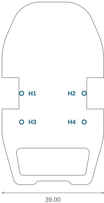
Full profile - viewed from top
