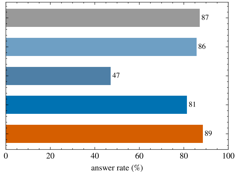
(b) SelfAware answerable (higher = better)
