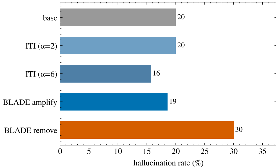
(a) SelfAware unanswerable (lower = better)
